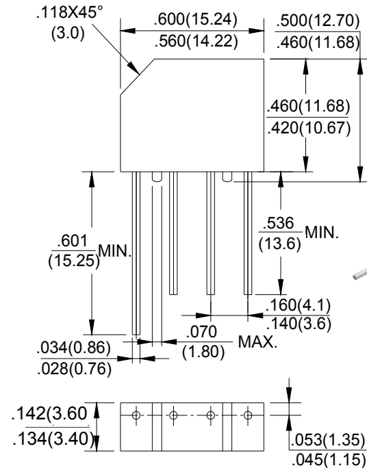
Package Outline Dimensions in Inches (Millimeters)
